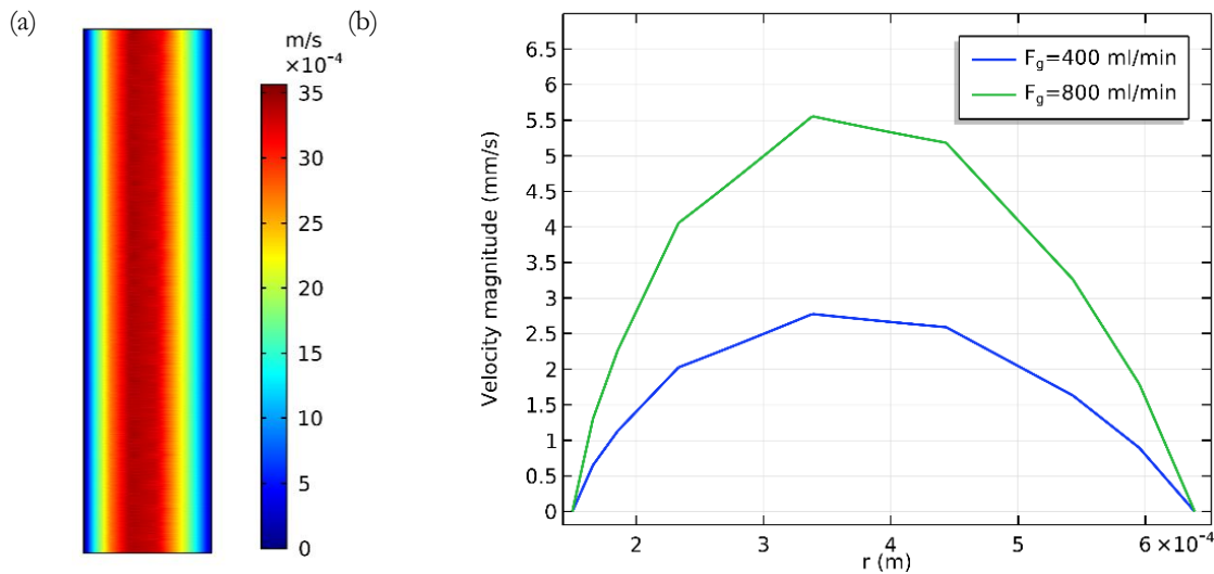
Figure 4. (a) The velocity profile in the shell side for F_g=500 \text{ ml/min} and (b) The parabolic velocity profile of the gas at z = 0 for the minimum ( 400 \text{ ml/min} ) and the maximum ( 800 \text{ ml/min} ) gas flow rates.
