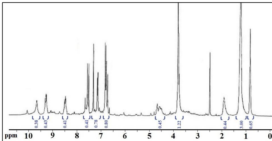
Fig. 4. ^1\text{H} NMR spectrum of CP in DMSO- d_6 .
