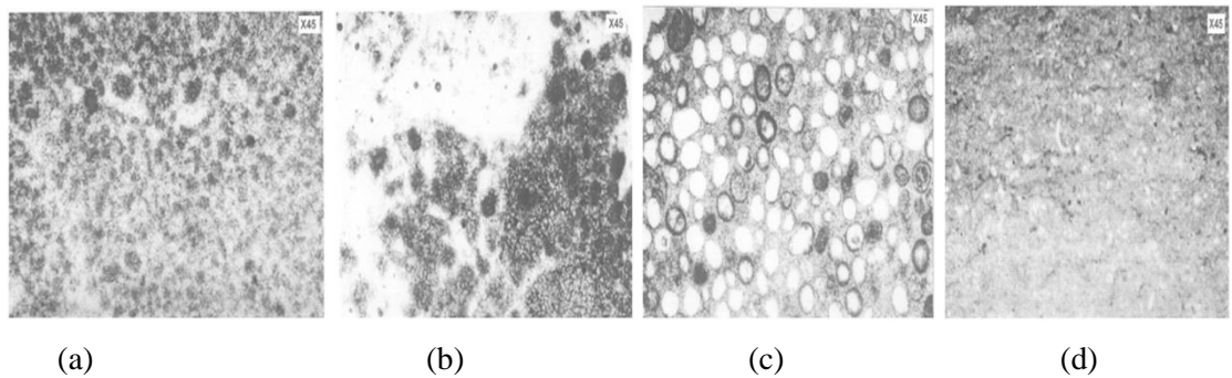
Figure 5: the samples taken from Kangan formation (a) in depth of 2136 m. with Dolomitized and Pelley lithology (b) in depth of 2149 m. with Pseudo-oolitic and Dolomitic lithology (c) in depth of 2157 m. with oolitic lithology, but Oolites are filled with Dolomite crystals (d) in depth of 2202 m. with lithology Mudstone, with small Ostracodes
