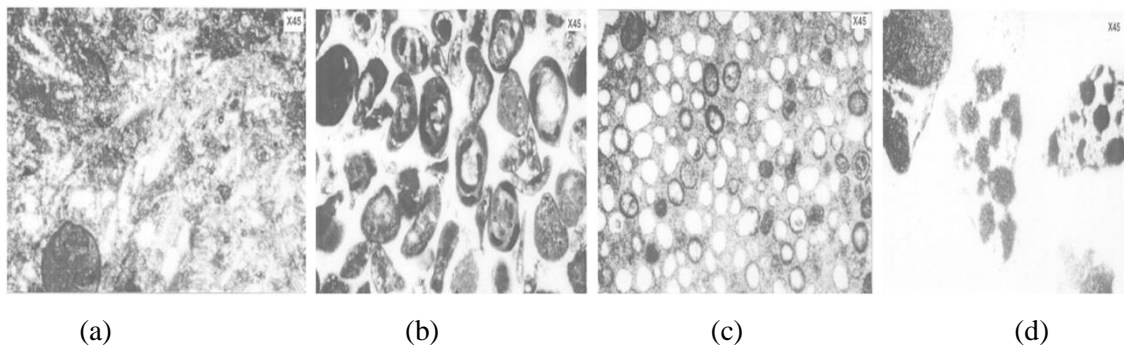
Figure 8: the samples taken from the substrate upper Dalan (a) in depth of 2319 m. with Wackstone, algae, and foraminifera lithology (b) in depth of 2322 m. with Packstone / Grainstone, Pseudo_Oolitic lithology (c) in depth of 2450 m. with Oolitic facies, with Oomoldic Porosity lithology (d) in depth of 2540 m. with Grainstone, Anhydritic lithology
