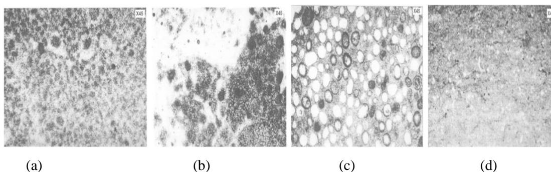
Figure 5: the samples taken from Kangan formation (a) in depth of 2136 m. with Dolomitized and Pellety lithology (b) in depth of 2149 m. with Pseudo-oolitic and Dolomitic lithology (c) in depth of 2157 m. with oolitic lithology, but Oolites are filled with Dolomite crystals (d) in depth of 2202 m. with lithology Mudstone, with small Ostracodes
