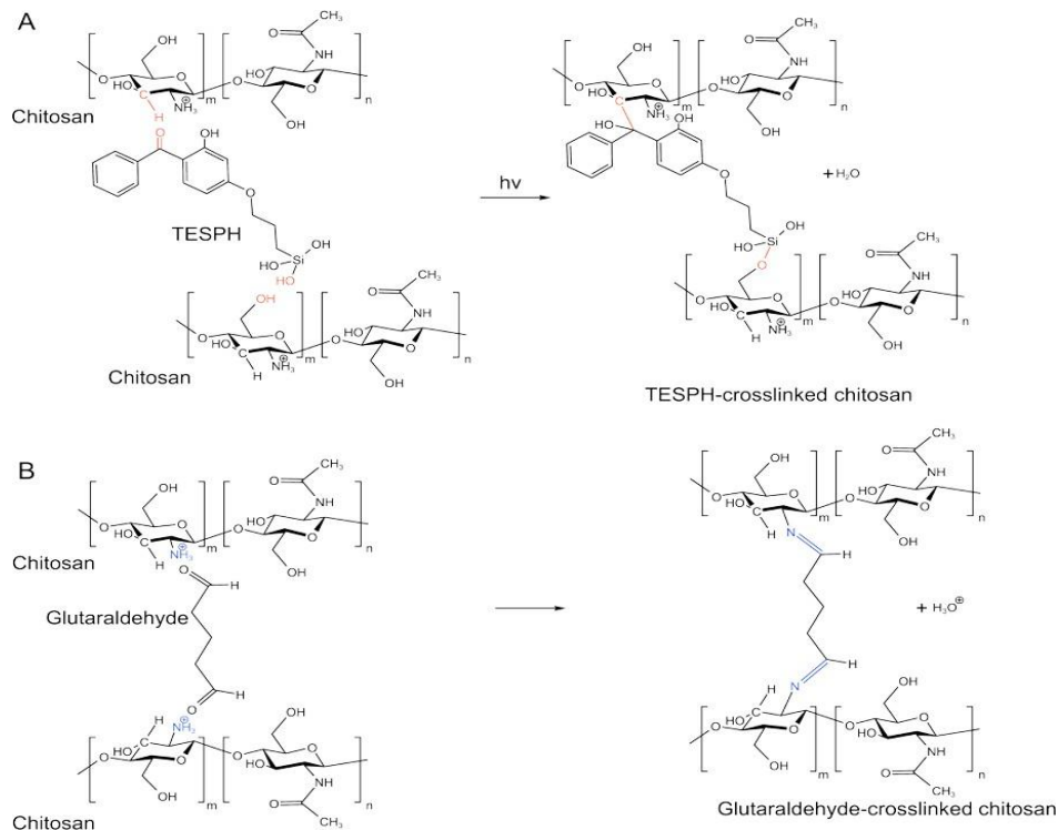
Figure 5. Reaction schemes of chitosan crosslinking by TESP and glutaraldehyde.
