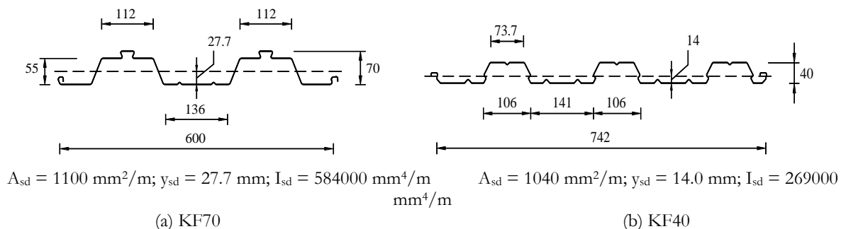
Figure 2. Dimensions (in mm) of each steel decking profile ( t_{sd}=0.75 mm)
