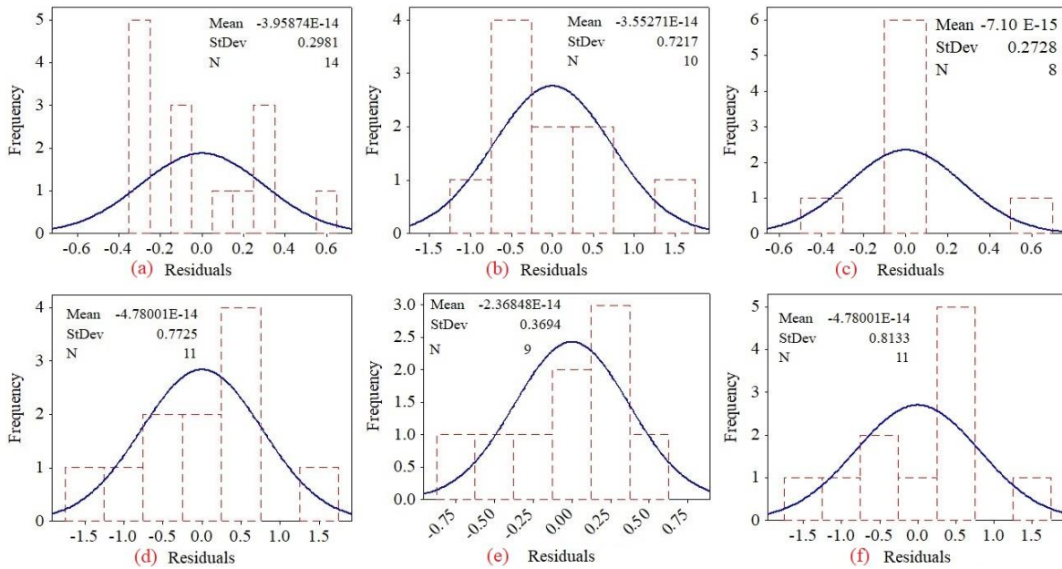
Figure 14. Frequency histogram and normal curve of two-variable regression residuals mechanical properties. Relationship between: (a) SDI_{1st} with UCS and E, (b) SDI_{2st} with BTS and E, (c) SDI_{1st} with BTS and V_{p-sat} , (d) SDI_{2st} with BTS and V_{p-sat} , (e) SDI_{1st} with BTS and V_{s-sat} and (f) SDI_{2st} with BTS and V_{s-sat}
