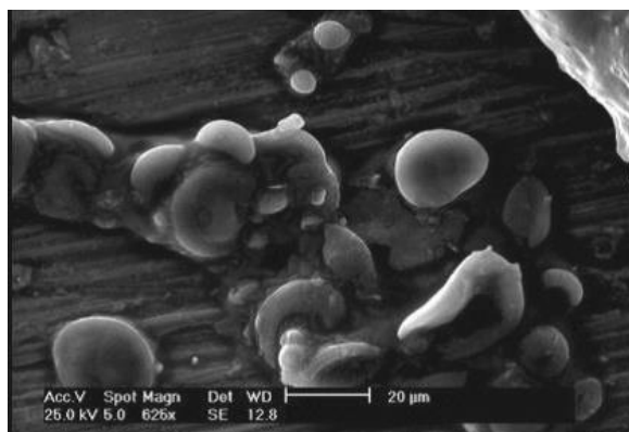
Figure 1. Spherical shape of Lambdacylhalothrin capsules by SEM
